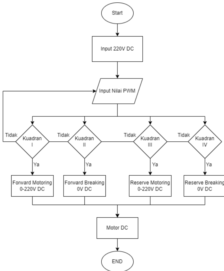
Figure 3. Flowchart system
