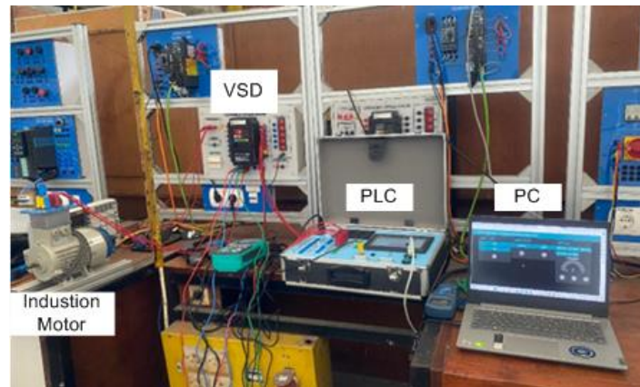
Figure 5. Hardware installation
