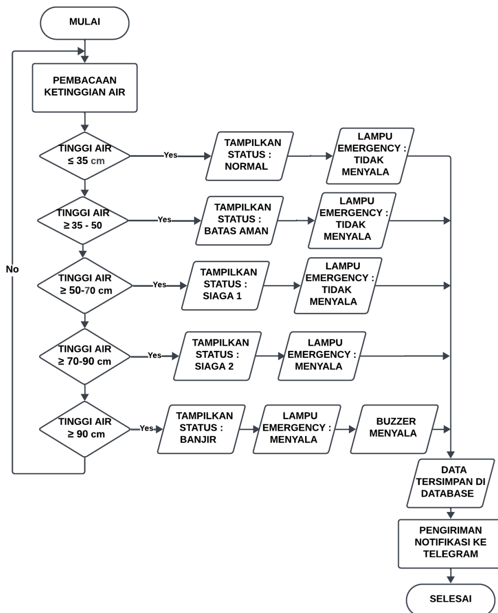
Figure 2. Flowchart of proposed system
