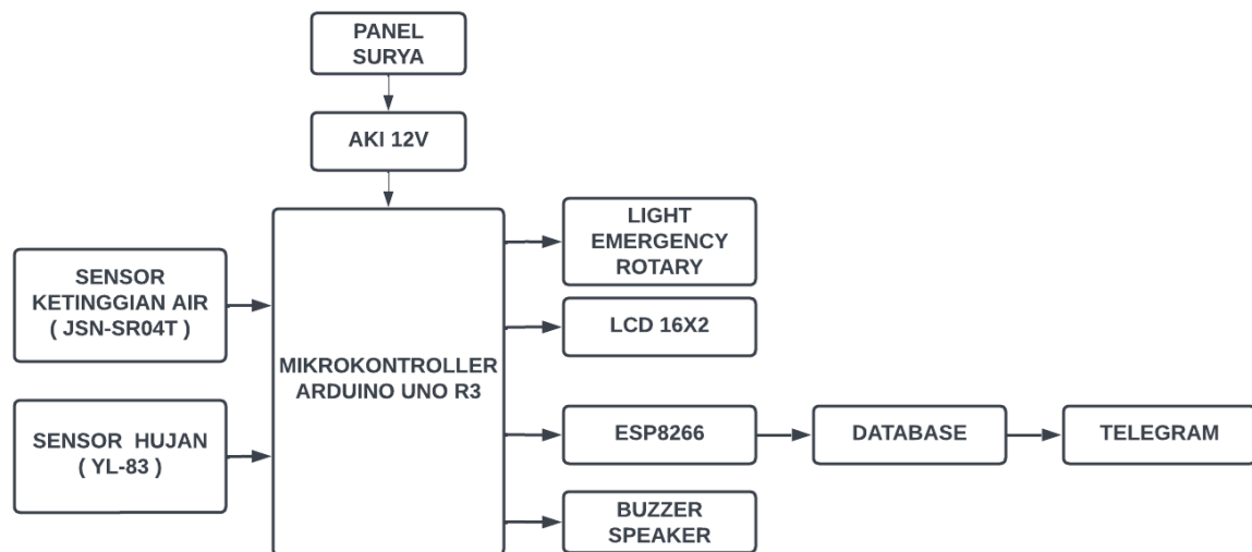
Figure 1. Diagram block of proposed system
