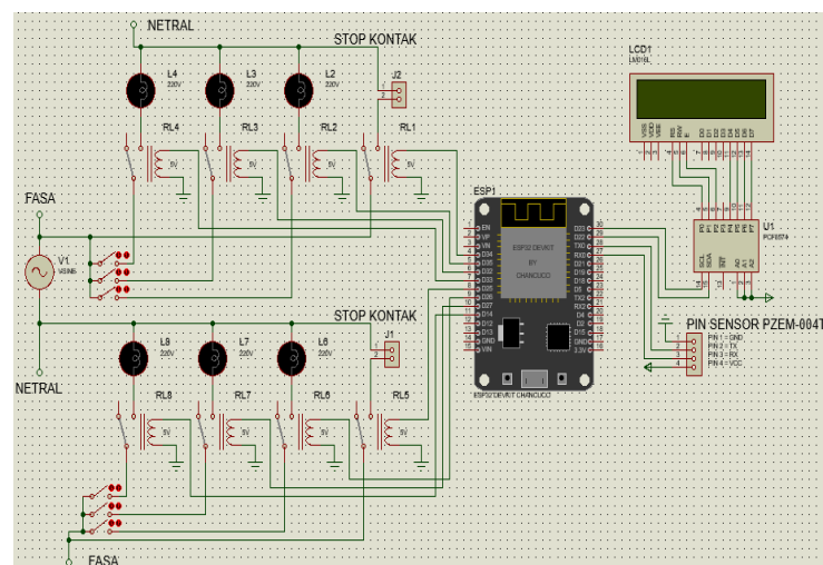
Figure 3. Circuit of monitoring and control system
