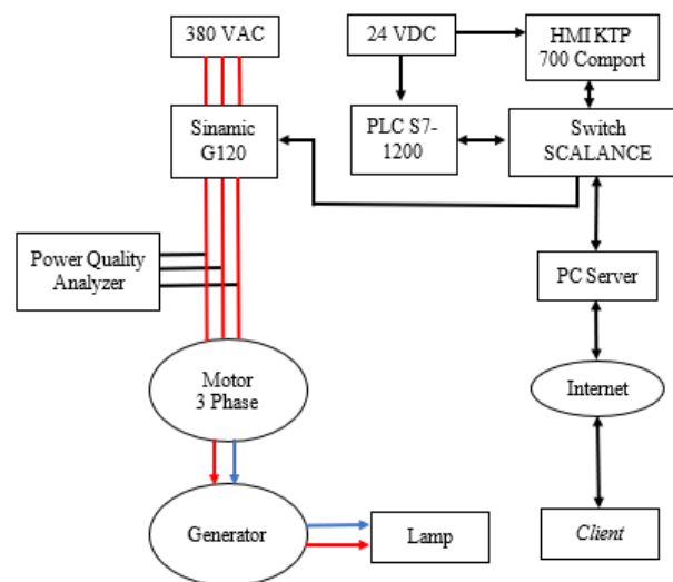
Figure 5. Experimental scheme
