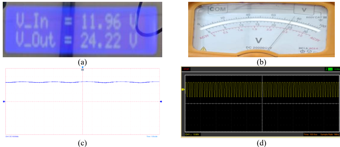
Figure 7. Experimental results with output voltage 24 Volt, (a) LCD, (b) Voltmeter, (c) Output voltage waveform in Oscilloscope, (d) PWM waveform at gate driver
