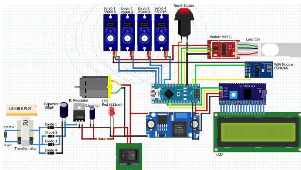
Figure 3. Circuit sheme
