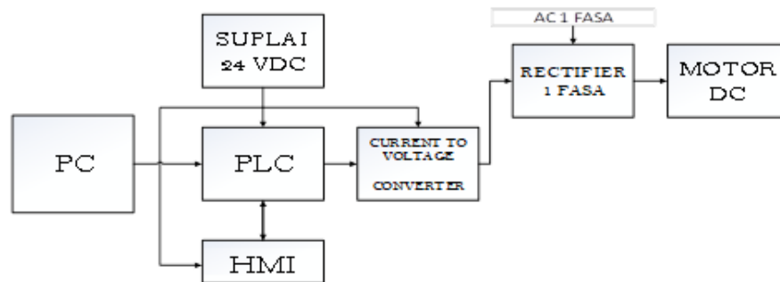
Figure 1. DC motor control block diagram
