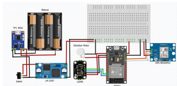
Figure 3. Control circuit of the proposed system
