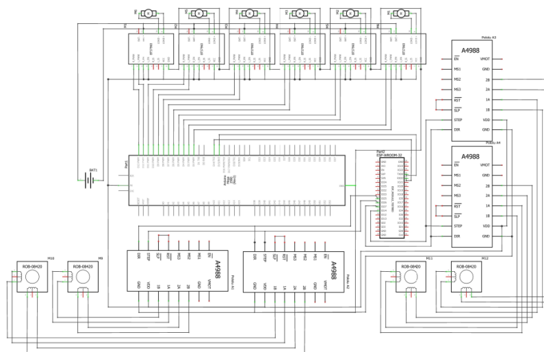
Figure 3. Robot electronics circuit
